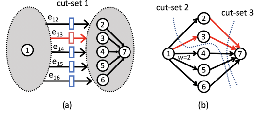
Figure 7: Assume that the edges e_{13} , e_{37} and e_{27} are pipelined according to some floorplan, and each of them carries 1 unit of inserted latency. Also assume that the bitwidth of e_{14} is 2 and all other edges are 1. In the latency balancing step, the optimal solution is adding 2 units of latency to each of e_{47} , e_{57} , e_{67} and 1 unit of latency to e_{12} . Note that edge e_{27} and e_{37} can exist in the same cut-set.
