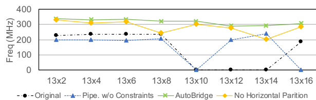
Figure 14: Control experiments with the CNN accelerators.
