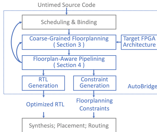
Figure 2: Overview of the AutoBridge Framework. Grey boxes represent the original software flow and blue boxes represent components of AutoBridge.
