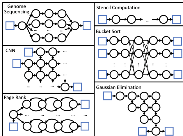
Figure 10: Topologies of the benchmarks. Blue rectangles represent external memory ports and black circles represent computation kernels of the design. In the genome sequencing design, the arrows represent BRAM channels; in other designs, the arrows represent FIFO channels.
