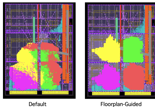
Figure 5: Implementation results of a stencil computing design on U280. Floorplanning during HLS compilation significantly benefits the physical design tools.
